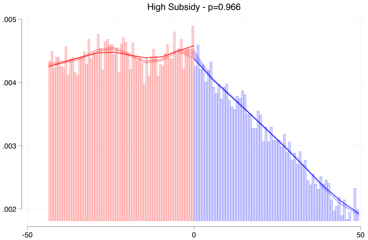
Figure 3: McCrary test after application
